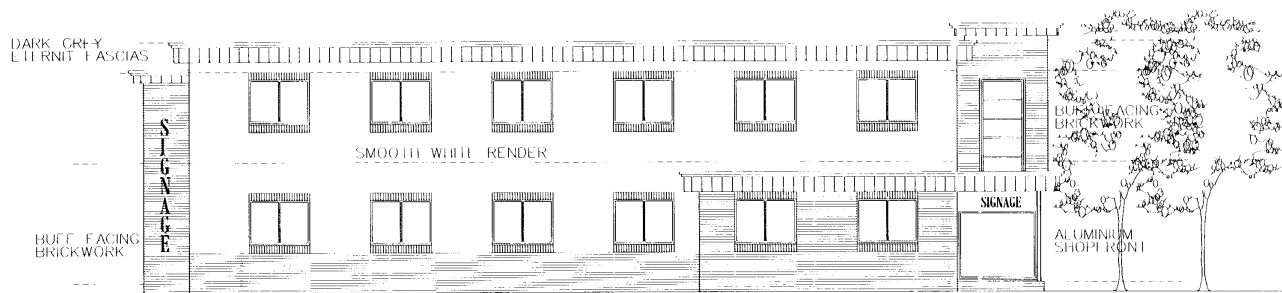
SOUTH ELEVATION
